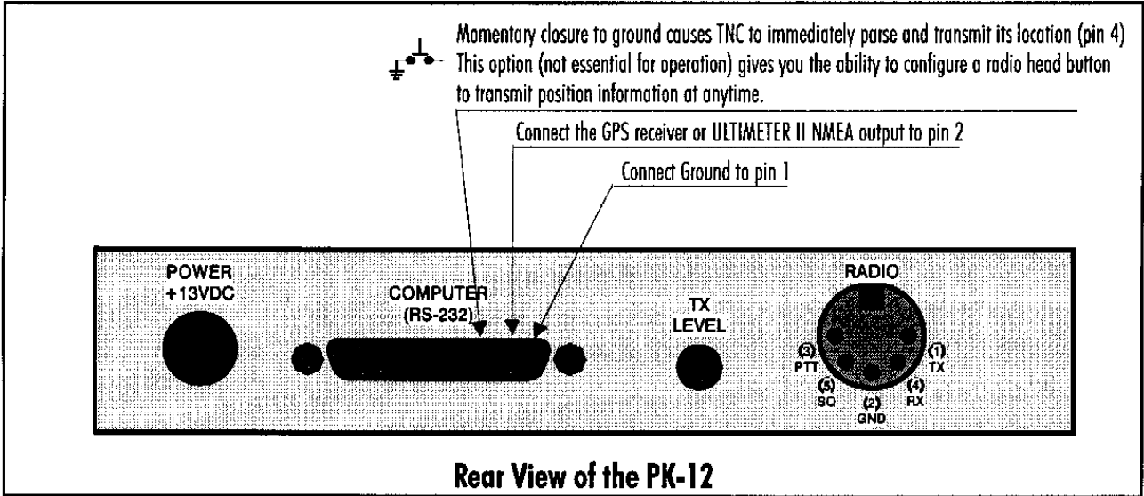
FIGURE 4: Pin assignments for connecting the TNC to a GPS receiver or to an Ultimeter II weather stations. (Same for all Timewave TNCs)
