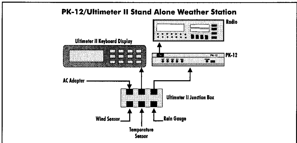
FIGURE 3: Illustrates components of a stand alone packet weather station (PK-12 can be substituted with any Timewave TNC with GPS firmware)
